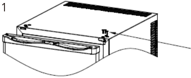
1 Removing the three right hinge fixing screws with a phillips screwdrive.
